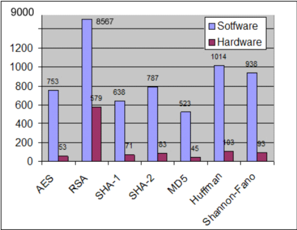
Fig. 5. Impact of the dedicates cores
