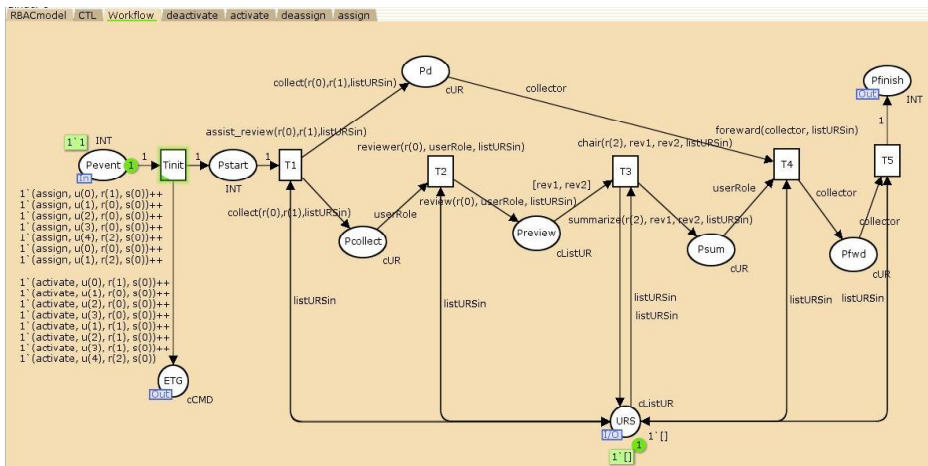
Fig. 11. CP-net representation of the paper review process
