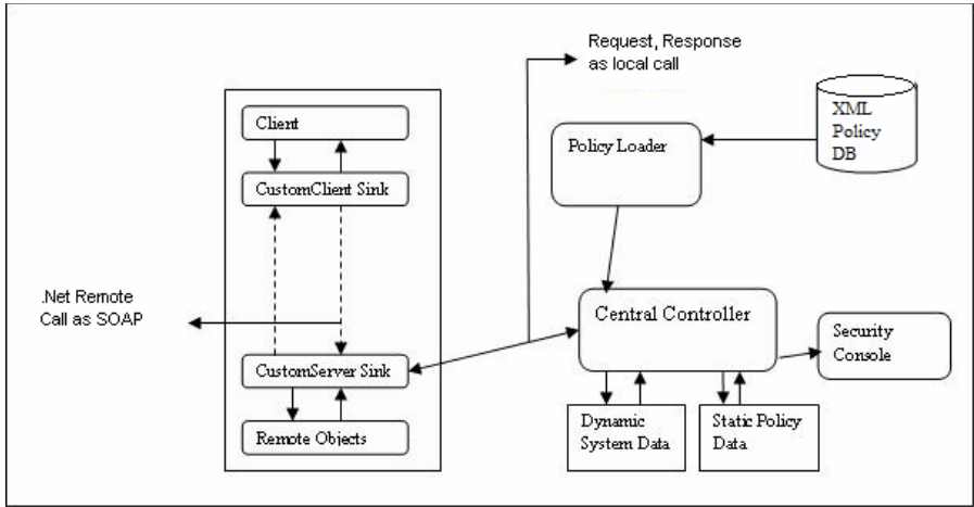
Fig. 3. Access Control System Architecture
