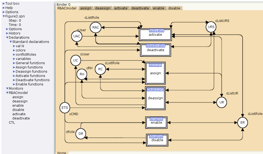
Fig. 2. CP-net representation of the RBAC model
