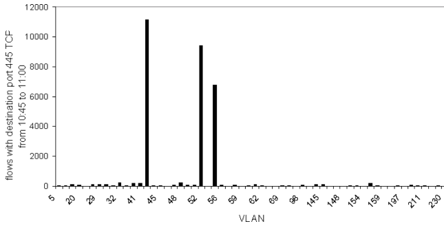
Fig. 5. Number of flows with destination port 445/TCP by VLAN from 10:45 to 11:00 on worm presence
