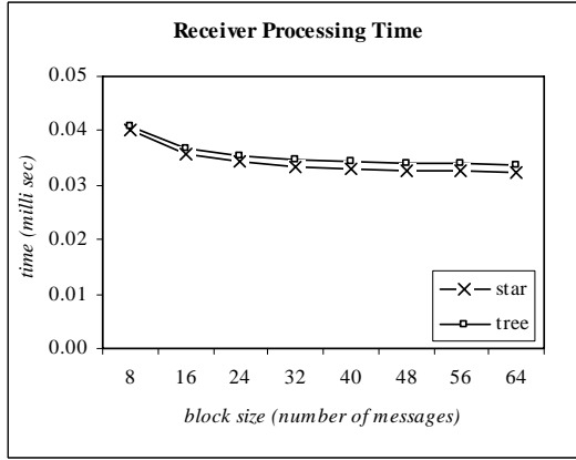
Fig. 7. Receiver processing time without forging
