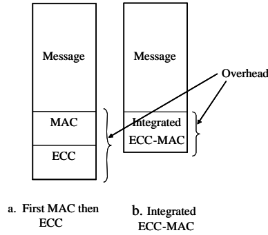
Fig. 2. Overhead for Conventional and Integrated Scheme
