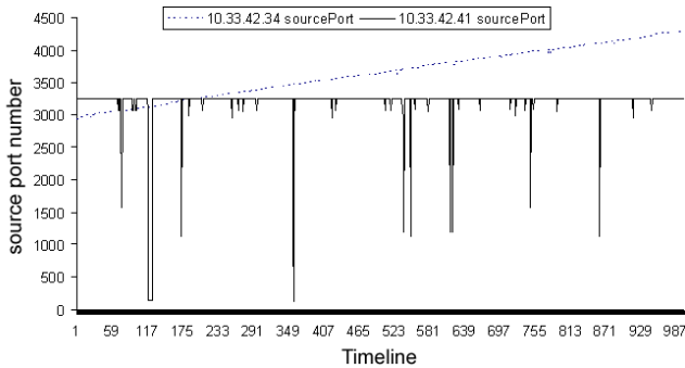
Fig. 7. Source Port organization in timeline
