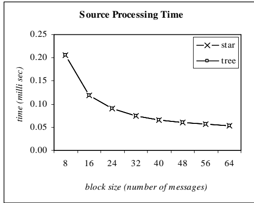
Fig. 6. Source processing time
