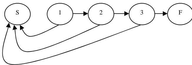
Fig. 2. The DNS spoofing attack modeling
