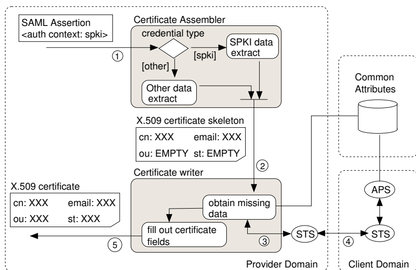
Fig. 3. Credential Translation Service
