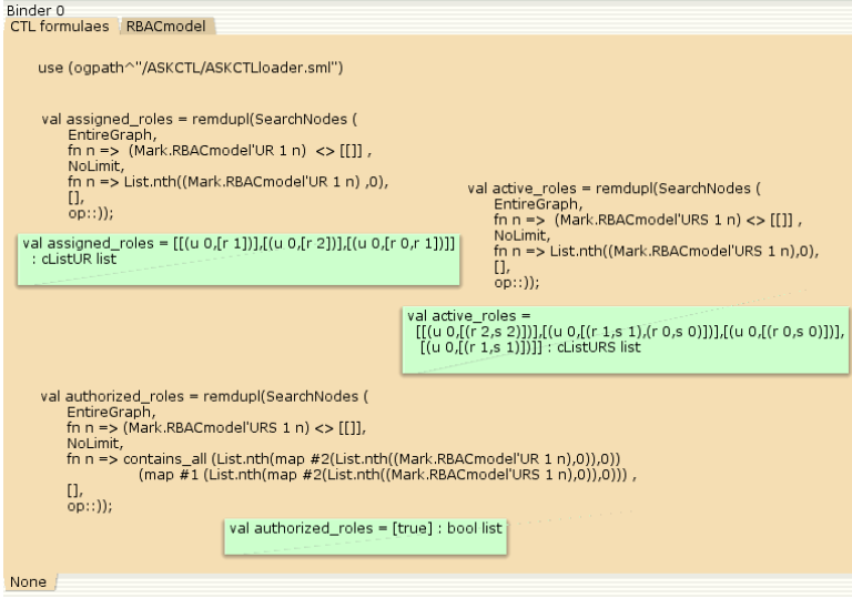
Fig. 8. Model-checking some RBAC consistency rules
