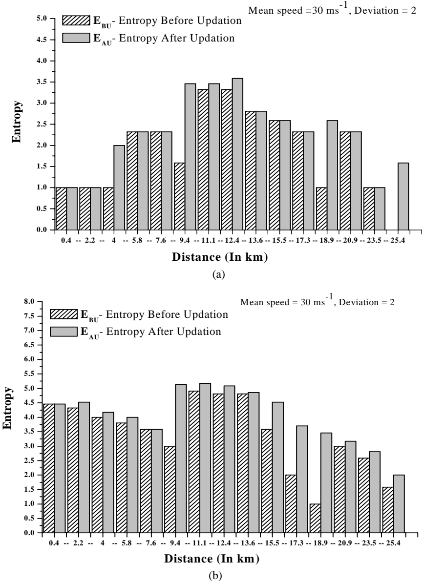
Fig. 3. (a) Entropy of the Vehicle of Interest (Transmission range = 100 m). (b) Entropy of the Vehicle of Interest (Transmission range = 500 m).
