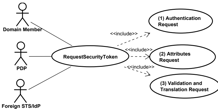
Fig. 5. Requests Handled by STS/IdP
