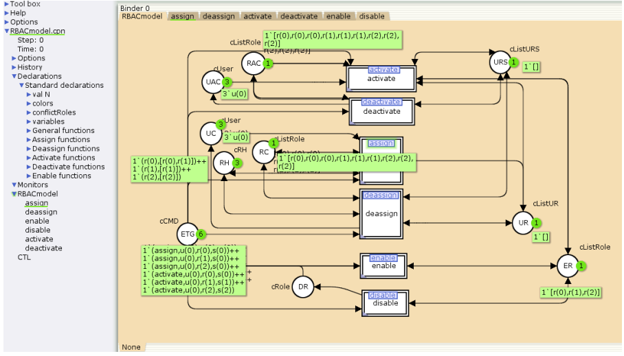
Fig. 6. Example of CP-net representation of an RBAC system
