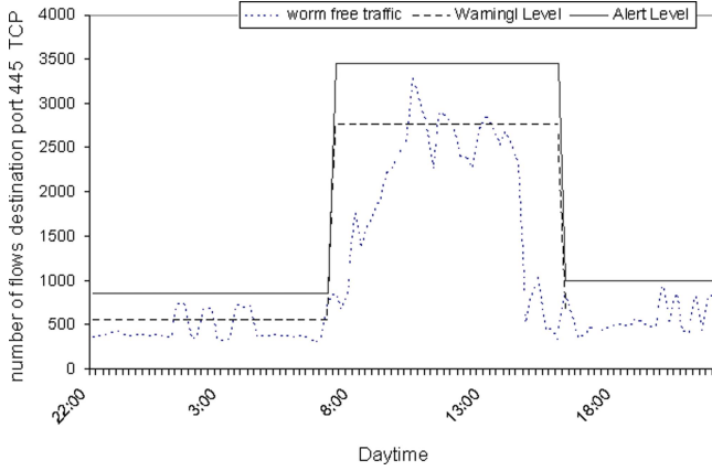
Fig. 3. Normalized flow levels to 445/TCP destination port in worm free status
