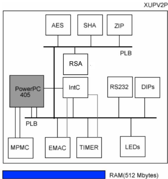
Fig. 2. Top-level architecture
