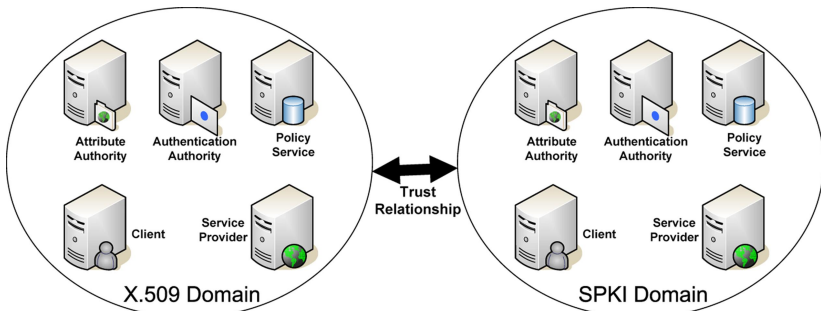
Fig. 1. Security Domains
