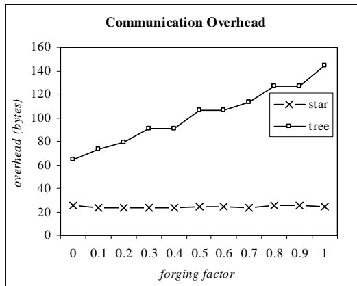
Fig. 10. Communication overhead with forging (maximum error probability = 0.5, and average error probability = 0.3)
