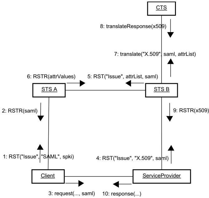
Fig. 7. UML Communication Diagram
