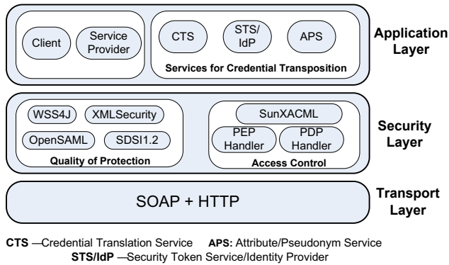
Fig. 4. Prototype Architecture
