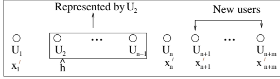
Fig. 4. Join operation
