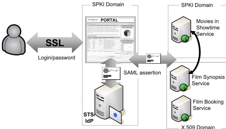
Fig. 6. Entertainment Portal
