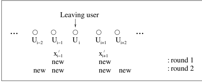
Fig. 5. Leave operation
