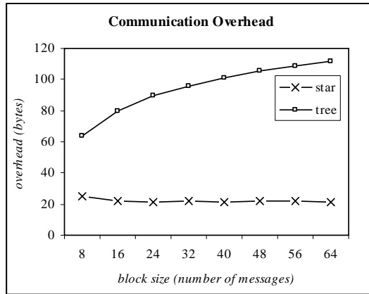
Fig. 9. Communication overhead
