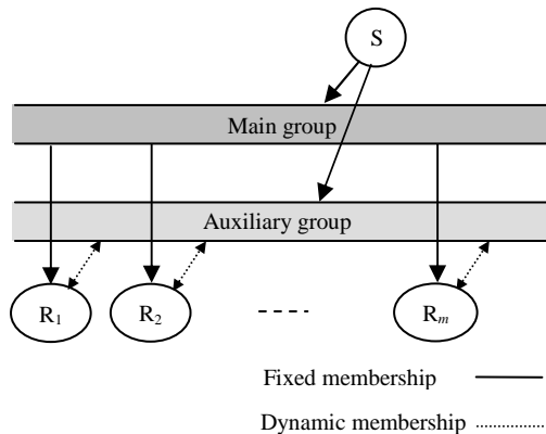
Fig. 2. Error control using two multicast groups
