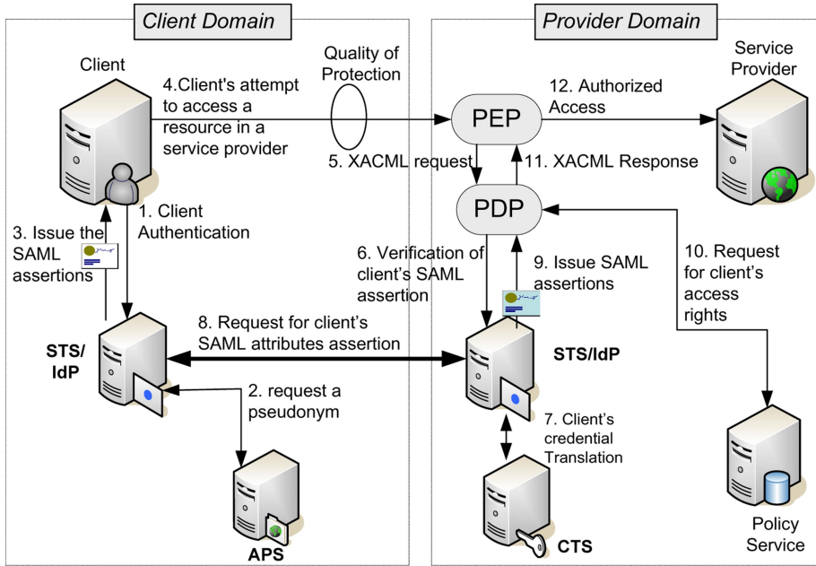
Fig. 2. Dynamics for Translation of Authentication Credentials
