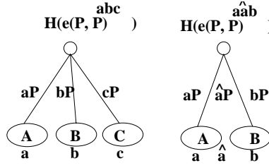
Fig. 1. procedure CombineThree and procedure CombineTwo
