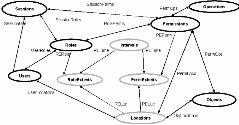
Fig. 1. Proposed ESTARBAC Model
