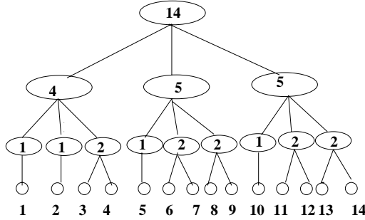
Fig. 2. procedure KeyAgreement for n = 14
