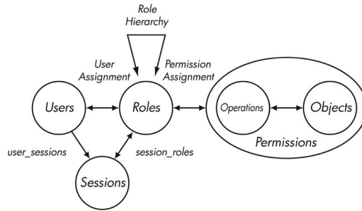
Fig. 1. The RBAC model
