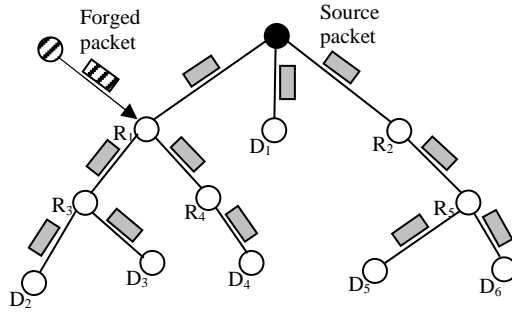
Fig. 5. Dropping forged messages in overlay multicast
