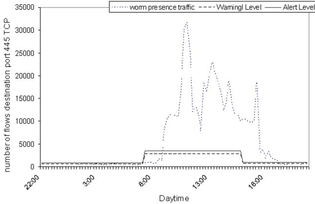
Fig. 4. Normalized 445 port flow number levels with worm infected hosts presence
