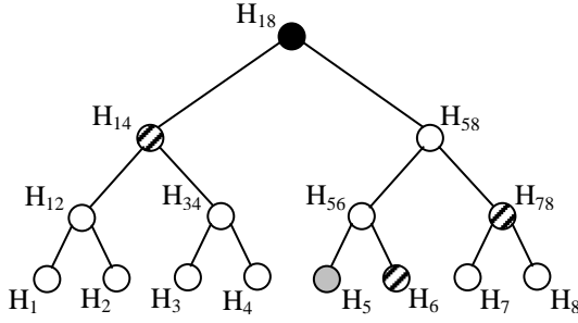
Fig. 1. Tree chaining signature amortization
