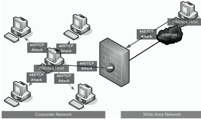
Fig. 1. Network scenario with the presence of an infected host
