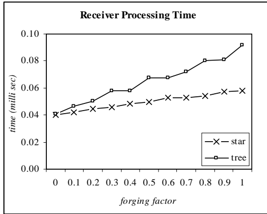
Fig. 8. Receiver processing time with forging
