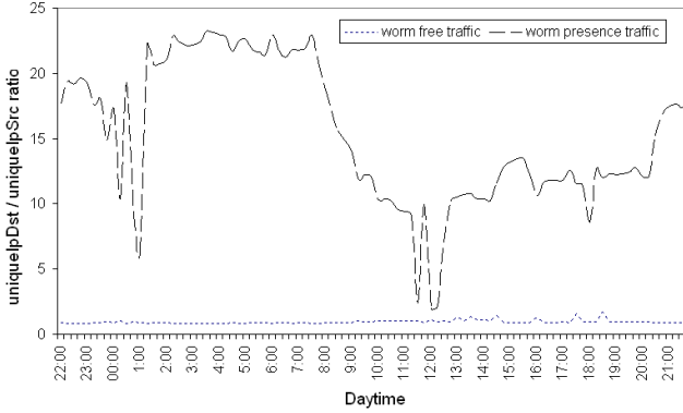
Fig. 6. Ratio of uniqueDestinationIp / uniqueSourceIp
