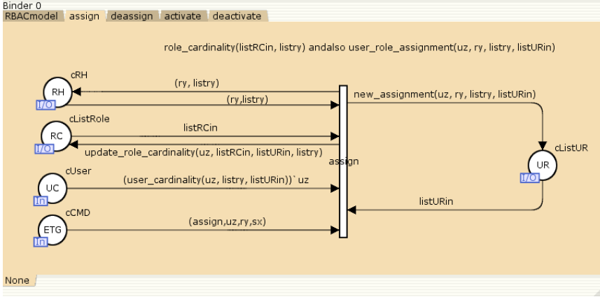
Fig. 5. CP-net construction for user-role assignment
