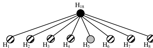
Fig. 3. Star chaining signature amortization
